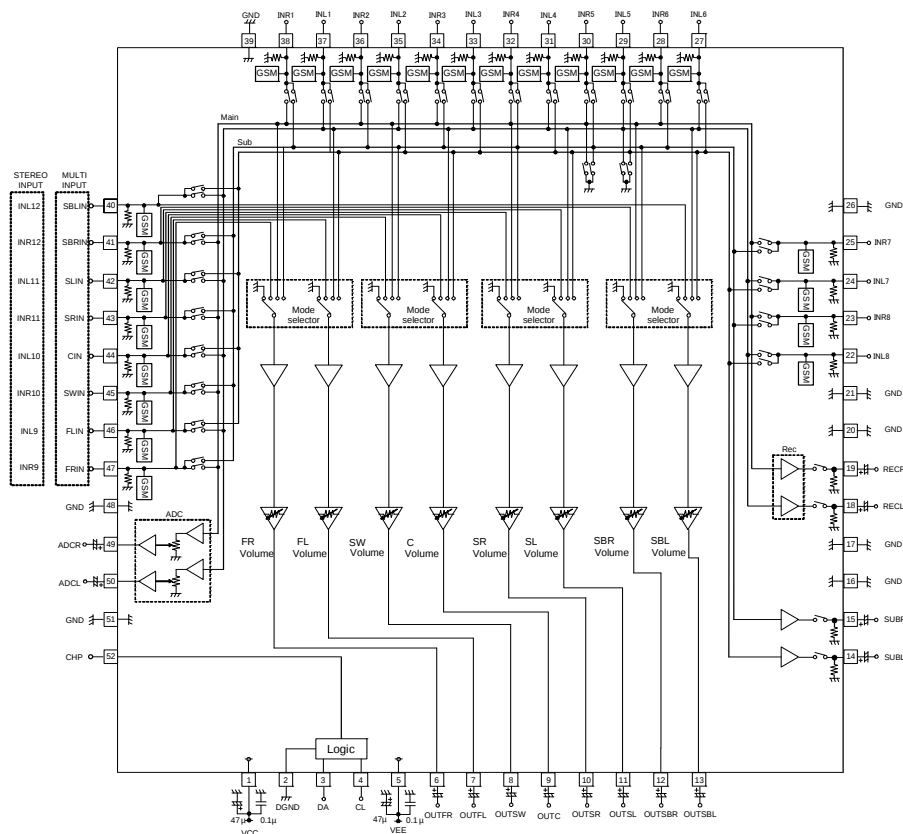
Figure 1. Application Circuit
