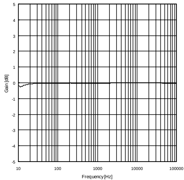
Figure 5. Gain vs Freq.
